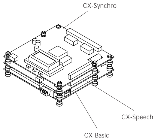
Mounting option with CX-Speech
