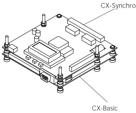
Mounting option without CX-Speech
